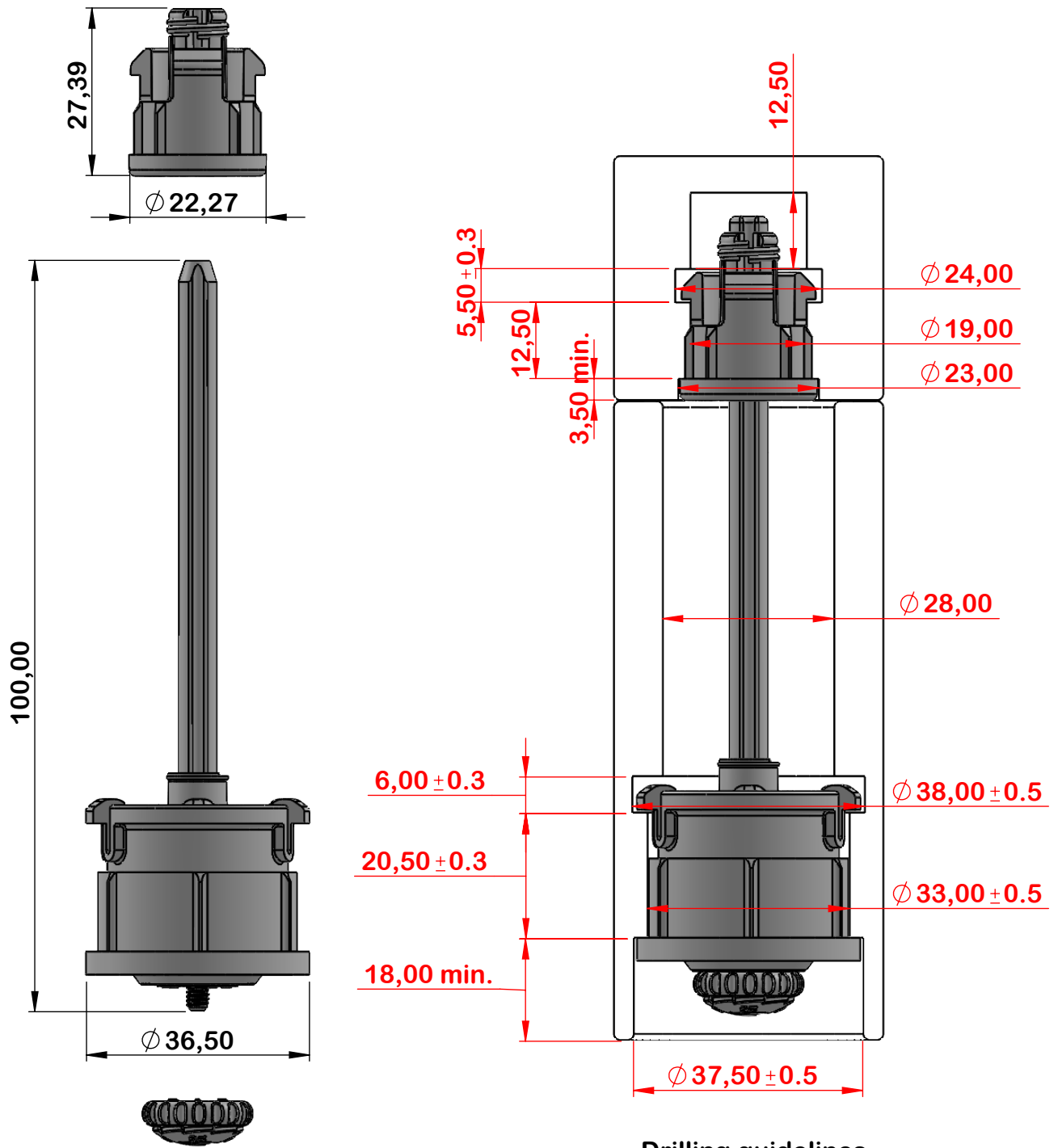
Drilling guidelines
